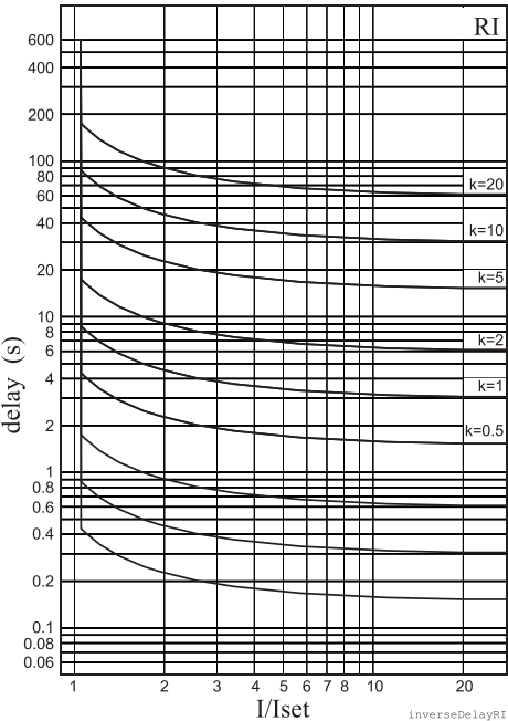
Figure 2.23.1-15 Inverse delay of type RI.
