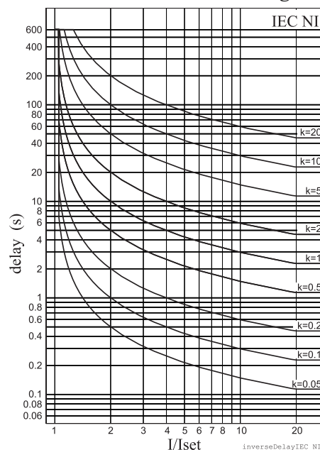
Figure 2.23.1-1 IEC normal inverse delay.
