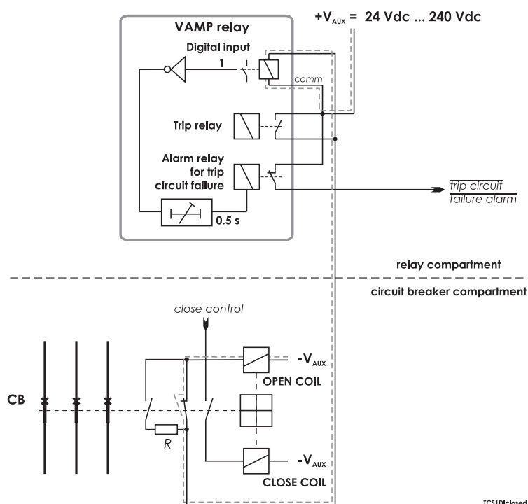
Figure 7.3.1-1 Trip circuit supervision using a single digital input and an external resistor R. The circuit-breaker is in the closed position. The supervised circuitry in this CB position is double-lined. The digital input is in active state when the trip circuit is complete.
