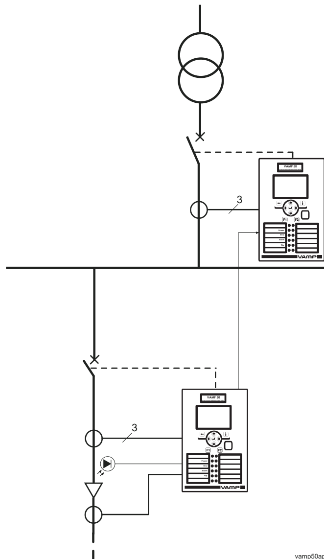
Figure 7.1-1 VAMP 50 or VAMP51 used in substation feeder protection
