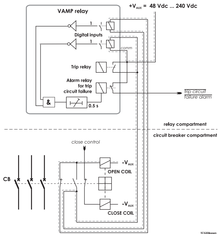
Figure 7.3.2-2 Trip circuit supervision with two digital inputs. The CB is in the open position. The two digital inputs are now in series.
