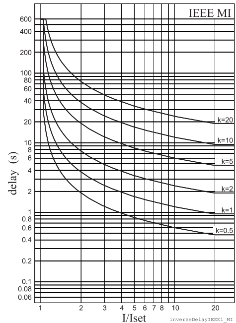
Figure 2.23.1-8 ANSI/IEEE moderately inverse delay
