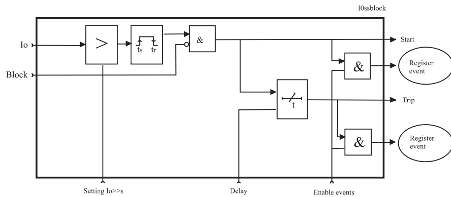
Figure 2-2 Block diagram of the earth fault stages I 0 >>, I 0 >>> and I 0 >>>>
