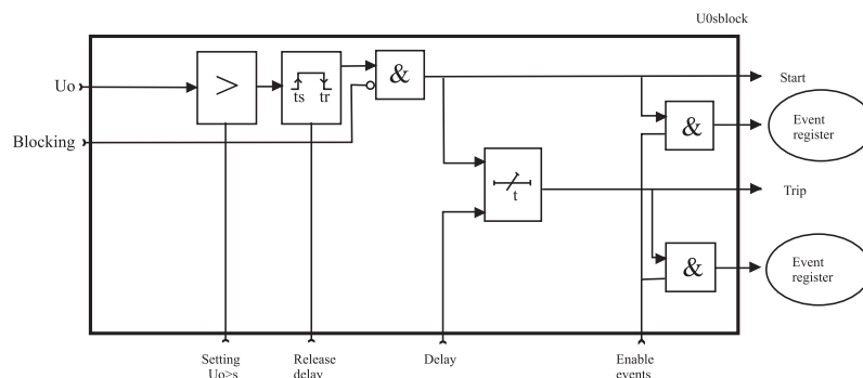
Figure 2.15-1. Block diagram of the zero sequence voltage stages U_0> and U_0>>
