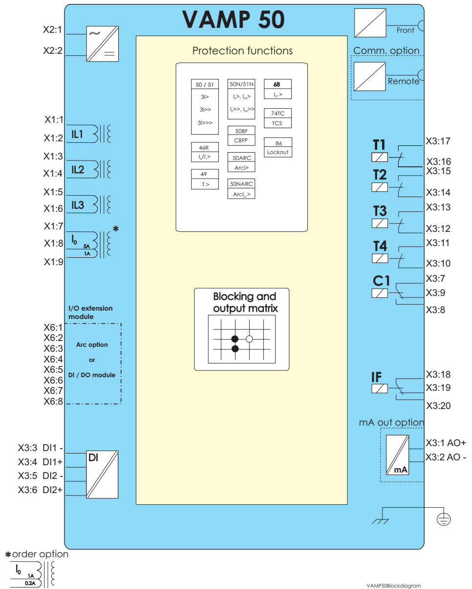
Figure 8.8.1-1. Block diagram of overcurrent and earthfault protection relay VAMP 50.
