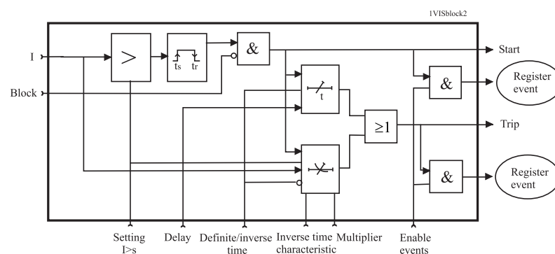
Figure 1.2-3 Block diagram of a basic protection function
