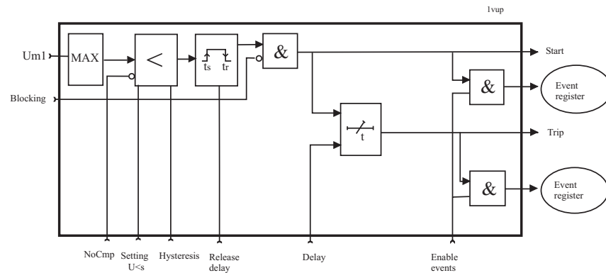
Figure 2.18-1 Block diagram of the single-phase undervoltage stages U<, U<< and U<<<
