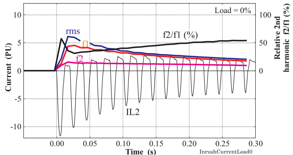
Figure 4-1 Example of various current values of a transformer inrush current.
