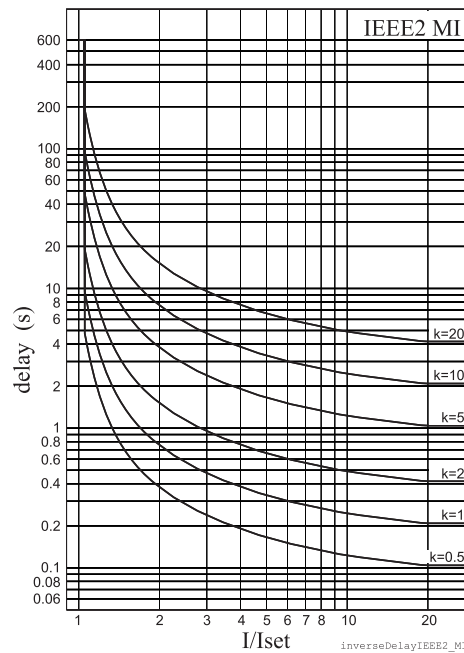
Figure 2.23.1-11 IEEE2 moderately inverse delay
