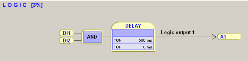
Figure 7.3.2-4 An example of logic configuration for trip circuit supervision with two dry digital inputs DI1 and DI2.
