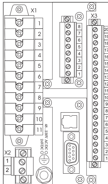
Figure 8.5-1 VAMP 50 with arc option card.
