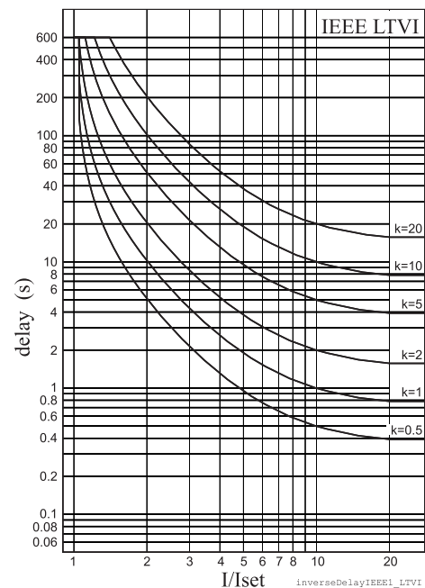
Figure 2.23.1-6 ANSI/IEEE long time very inverse delay
