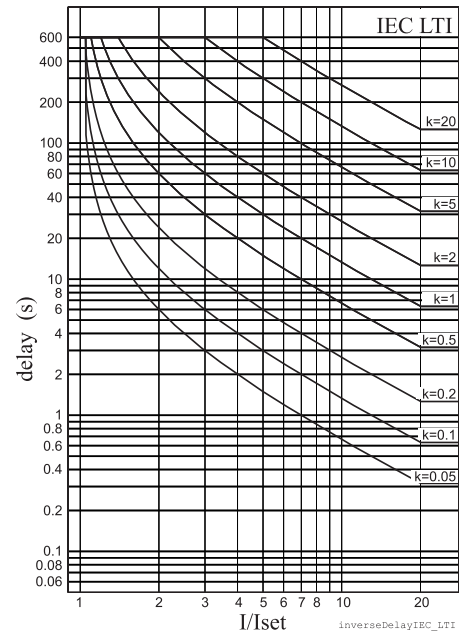
Figure 2.23.1-4 IEC long time inverse delay.
