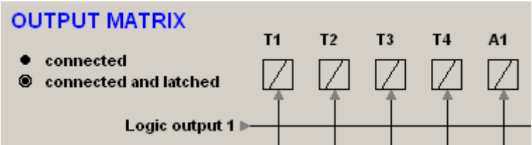
Figure 7.3.2-5 An example of output matrix configuration for trip circuit supervision with two digital inputs.
