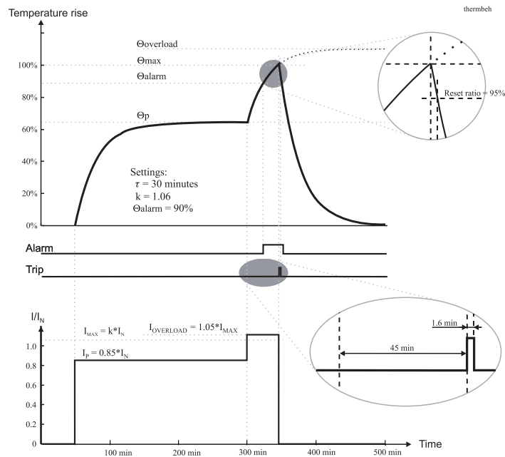
Figure 2.16-2. Example of the thermal model behaviour.
