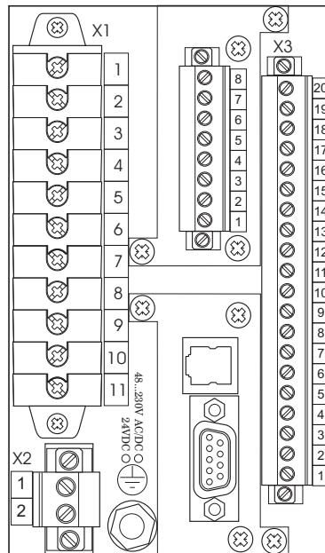
Figure 8.6-1 VAMP 50 with digital input/output option card.
