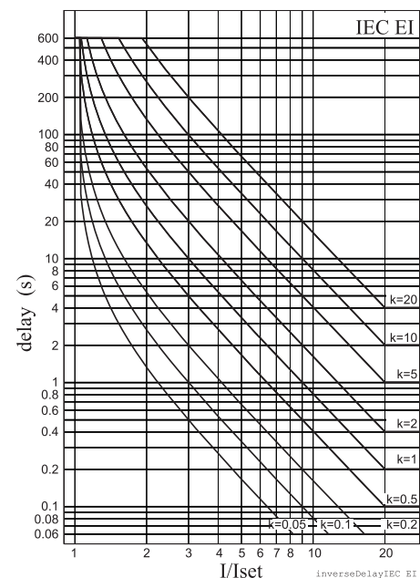
Figure 2.23.1-2 IEC extremely inverse delay.
