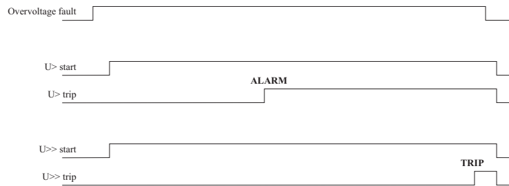
Figure 2.17-1 Settable start delay is obtained by combining two protection stages
