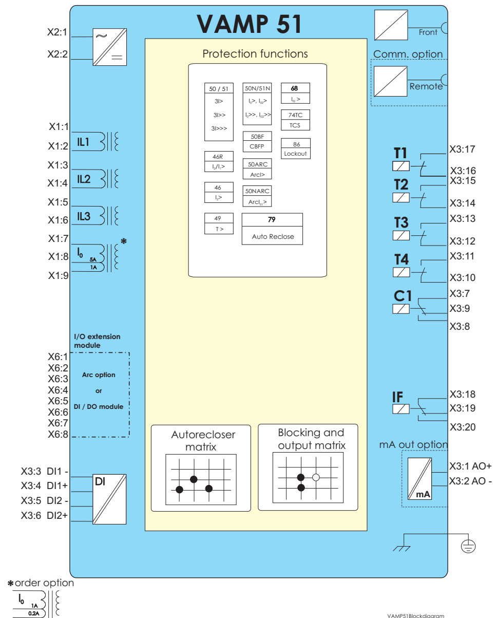
Figure 8.8.2-1 Block diagram of overcurrent and earthfault protection relay VAMP 51.
