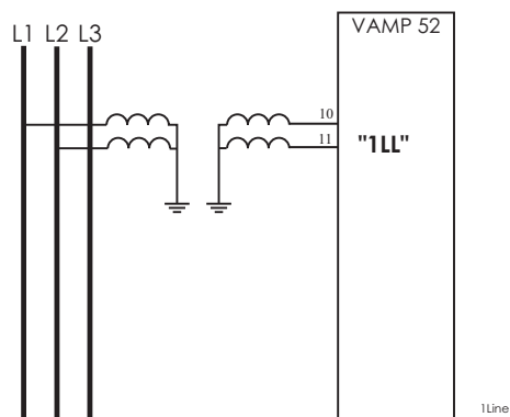
Figure 4.7-2 VAMP 52 line-to-line voltage in voltage measurement mode "1LL".
