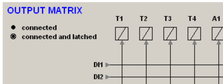
Figure 7.3.1-4 An example of output matrix configuration for trip circuit supervision with one digital input.
