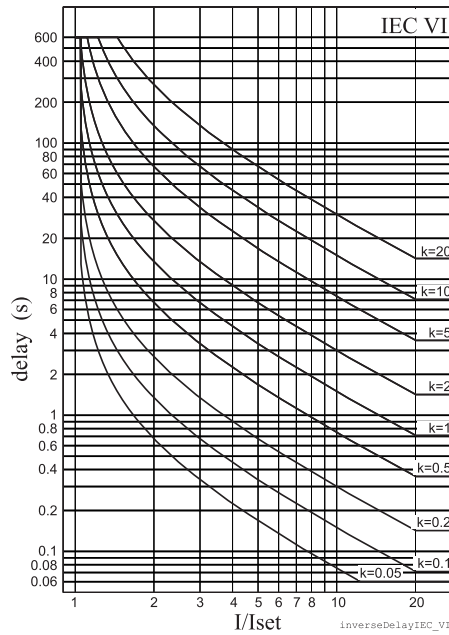
Figure 2.23.1-3 IEC very inverse delay.
