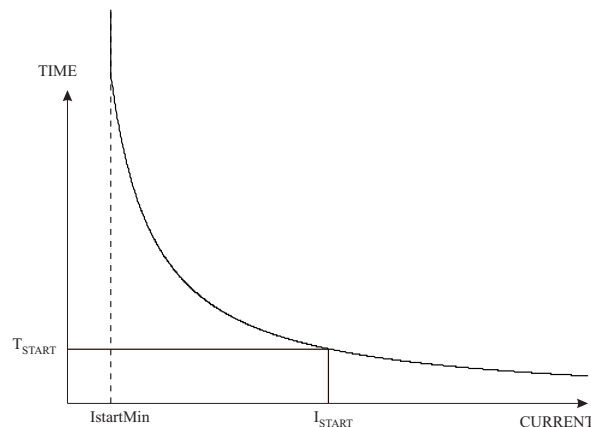
Figure 2.9-1 Operation time delay of the stall protection stage I_{st}> .
