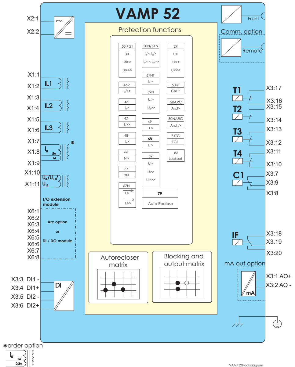
Figure 8.8.3-1 Block diagram of feeder/motor protection relay VAMP 52.
