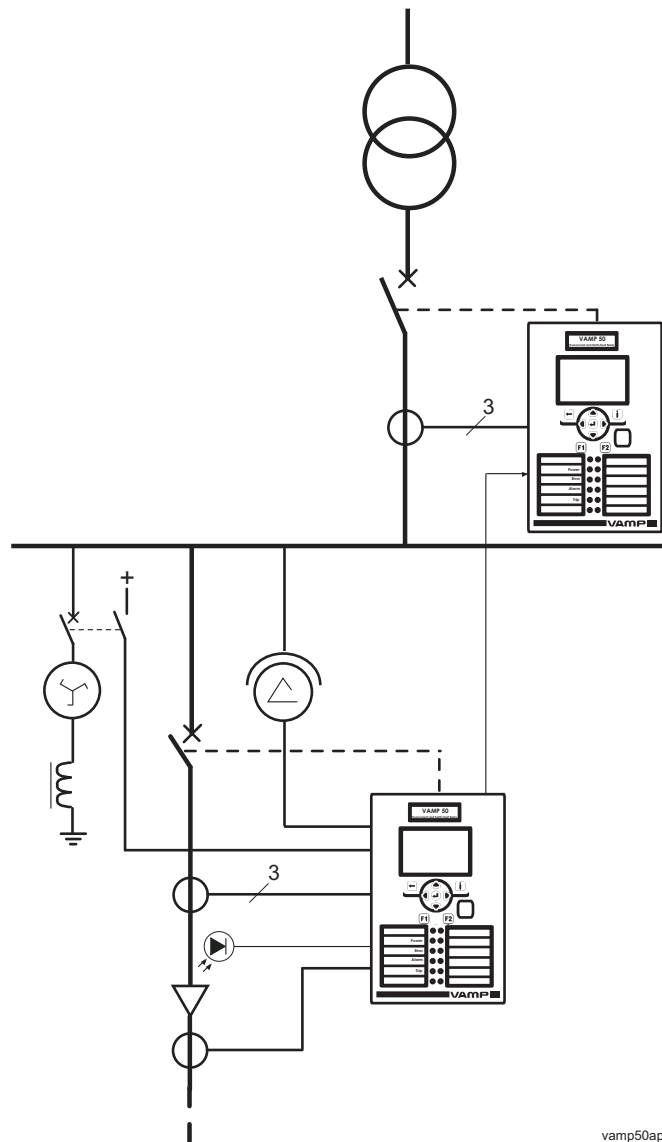
Figure 7.1-2 VAMP 52 used in substation feeder protection in compensated network
