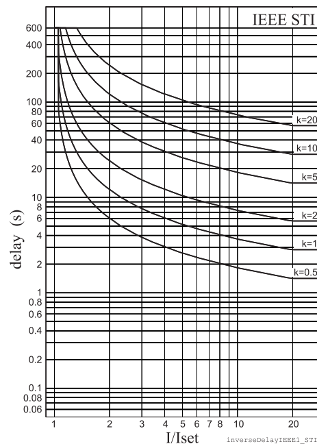
Figure 2.23.1-9 ANSI/IEEE short time inverse delay
