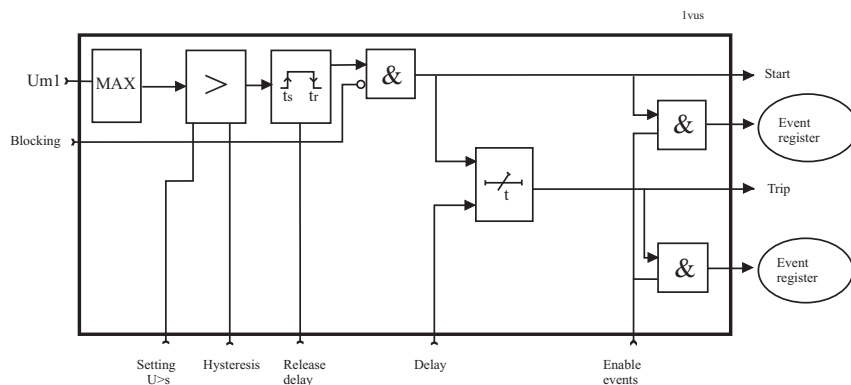
Figure 2.17-2 Block diagram of the single-phase overvoltage stages U>, U>> and U>>>
