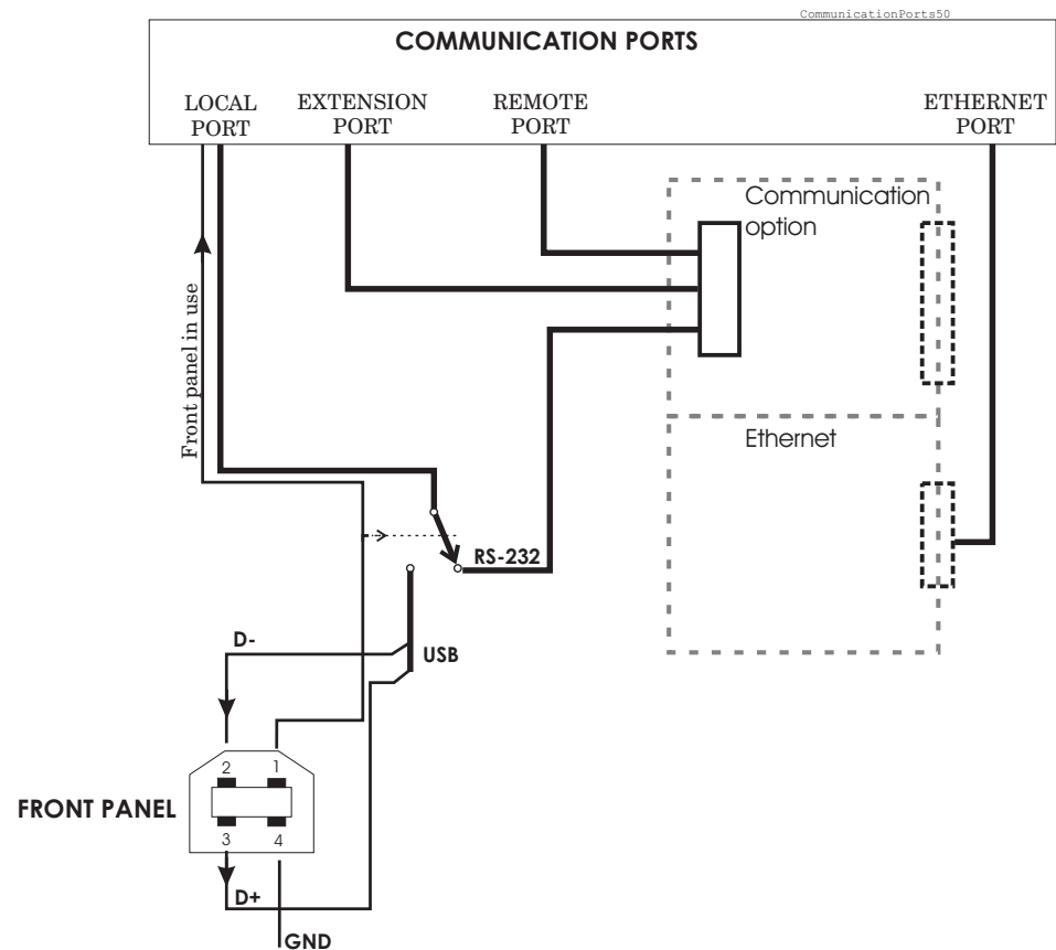
Figure 6.1-1. Communication ports and connectors. The DSR signal from the front panel port selects the active connector for the RS232 local port.
