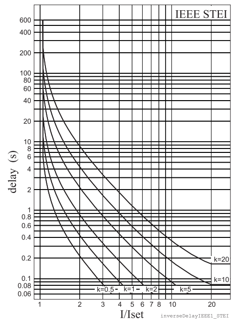
Figure 2.23.1-10 ANSI/IEEE short time extremely inverse delay
