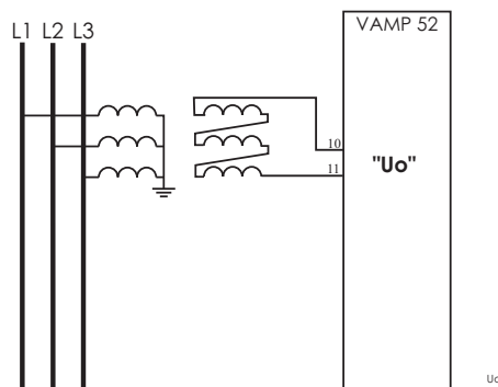
Figure 4.7-1 VAMP 52 Broken delta connection in voltage measurement mode "U o ".
