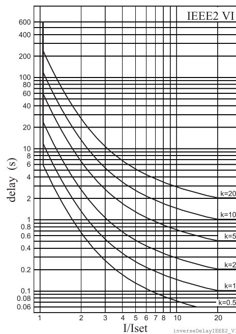
Figure 2.23.1-13 IEEE2 very inverse delay
