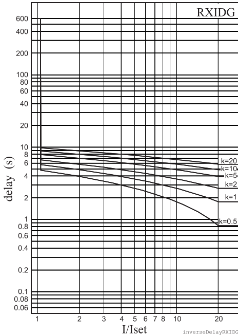
Figure 2.23.1-16 Inverse delay of type RXIDG.
