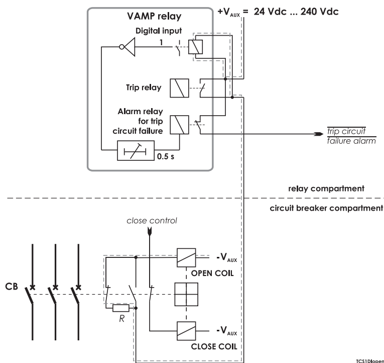
Figure 7.3.1-2 Trip circuit supervision using a single digital input, when the circuit breaker is in open position.
