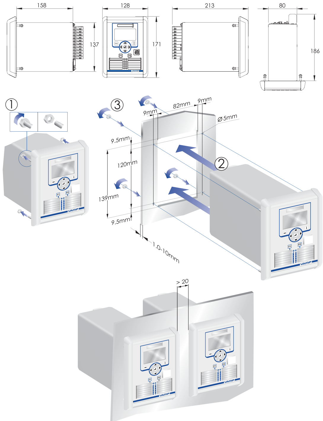
Figure 11-1 panel cut-out dimensions and Dimensional drawing
