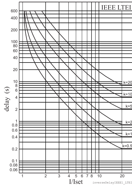
Figure 2.23.1-7 ANSI/IEEE long time extremely inverse delay
