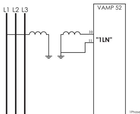
Figure 4.7-3 VAMP 52 phase-to-neutral voltage in voltage measurement mode "1LN".
