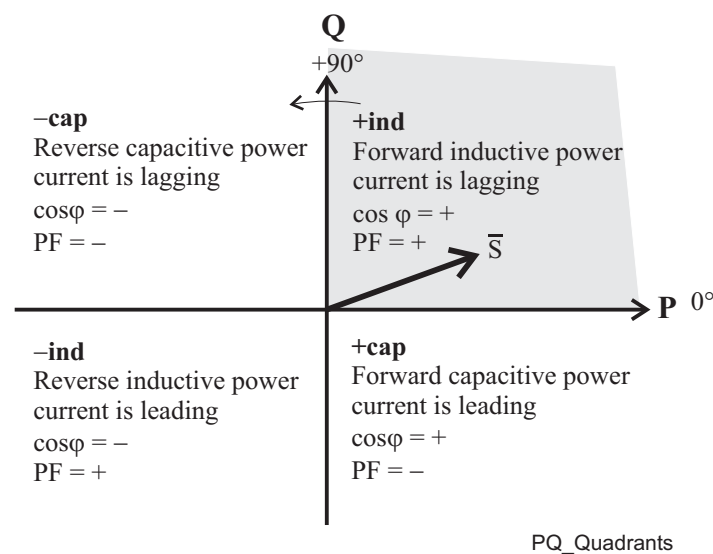
Figure 4.9-2 Quadrants of power plane
