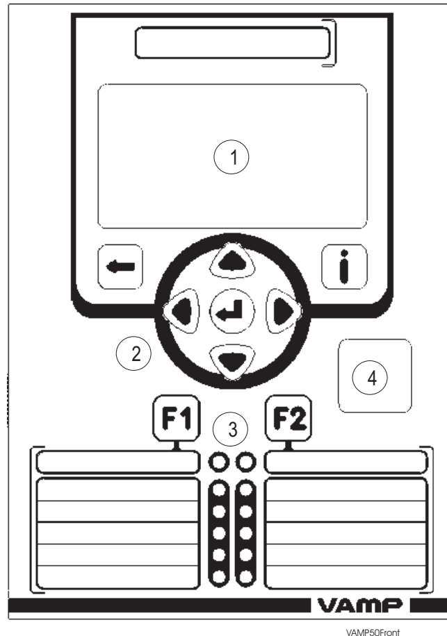
Figure 2.1-1. Relay front panel
