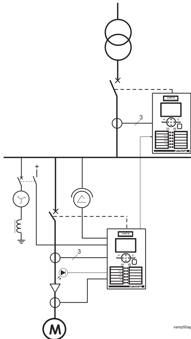
Figure 7.2-1 VAMP 52 feeder/motor protection relay used in cable protection of an industry plant network
