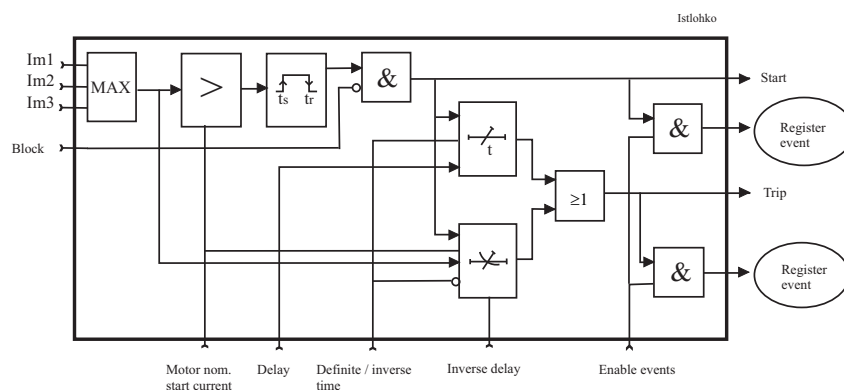
Figure 2.9-2 Block diagram of the stall protection stage I_{st}> .
