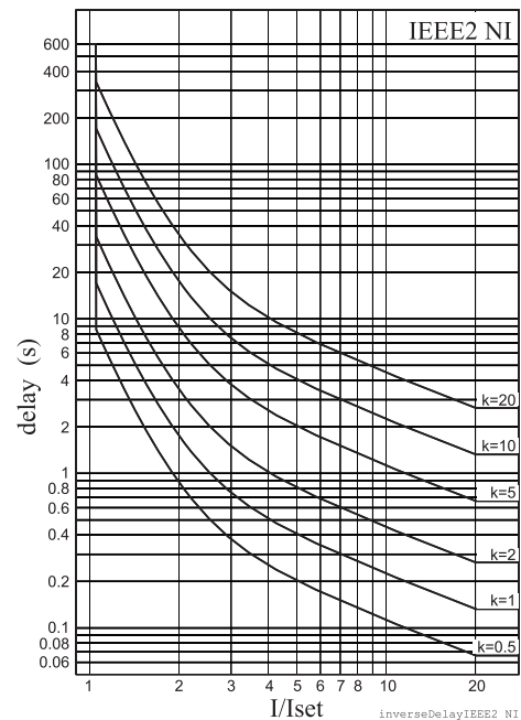
Figure 2.23.1-12 IEEE2 normal inverse delay
