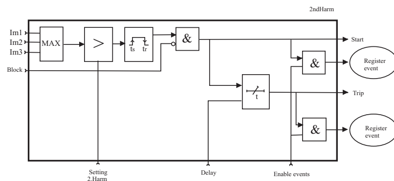
Figure 2.19-1 Block diagram of the second harmonic stage.
