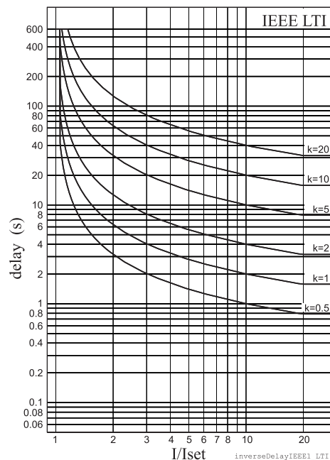
Figure 2.23.1-5 ANSI/IEEE long time inverse delay
