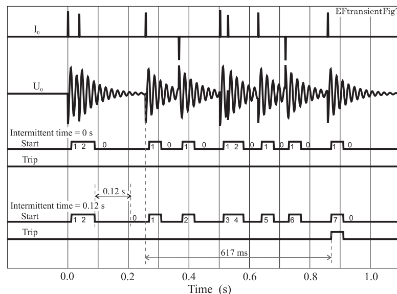
Figure 2.14-2. Effect of the intermittent time parameter. The operation delay setting is 0.14 s = 7x20 ms. The upper start and trip status lines are for a case with the intermittent time set to zero. No trip will happen. The lower start and trip status lines show another case with intermittent time setting 0.12 s. In this case a trip signal will be issued at t=0.87 s.
