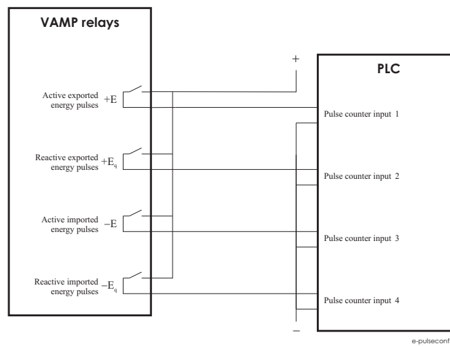
Figure 3.6-3. Application example of wiring the energy pulse outputs to a PLC having common minus and using an external wetting voltage
