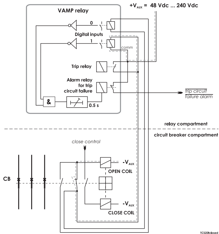
Figure 7.3.2-1 Trip circuit supervision with two digital inputs. The CB is closed. The supervised circuitry in this CB position is double-lined. The digital input is in active state when the trip circuit is complete.
