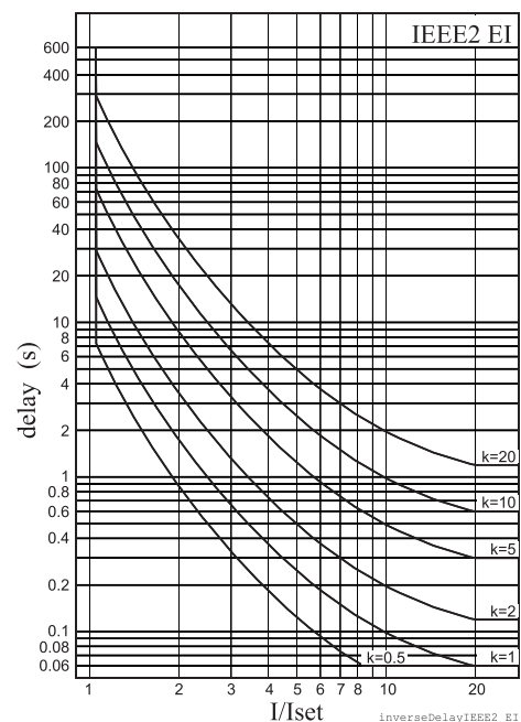
Figure 2.23.1-14 IEEE2 extremely inverse delay
