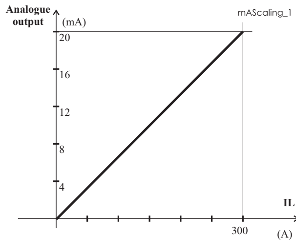
Figure 4.12.1-1. Example of mA scaling for IL, average of the three phase currents. At 0 A the transducer output is 0 mA, at 300 A the output is 20 mA
