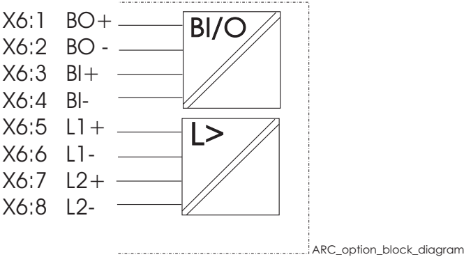
Figure 8.9-1Block diagram of optional arc protection card.
