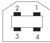
Figure 8-1 Pin numbering of the front panel USB type B connector
