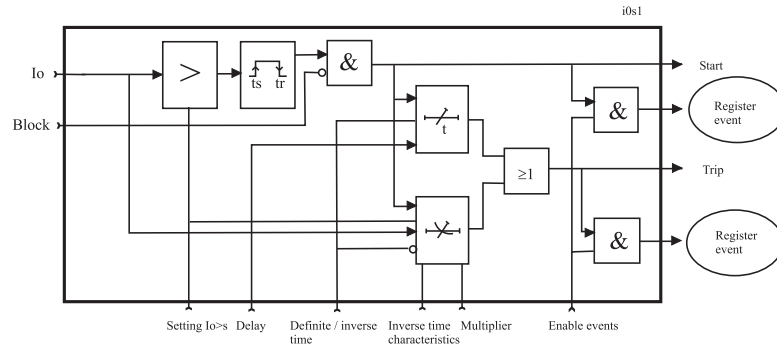
Figure 2-1 Block diagram of the earth fault stage I 0 >
