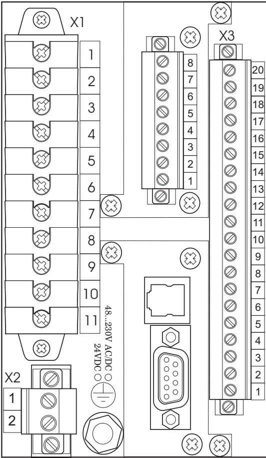
Figure 8.1-1 Connections on the rear panel of the VAMP 50, VAMP 51 and VAMP 52.
